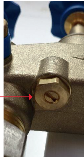
Slotted screw for residual hardness adjustment
